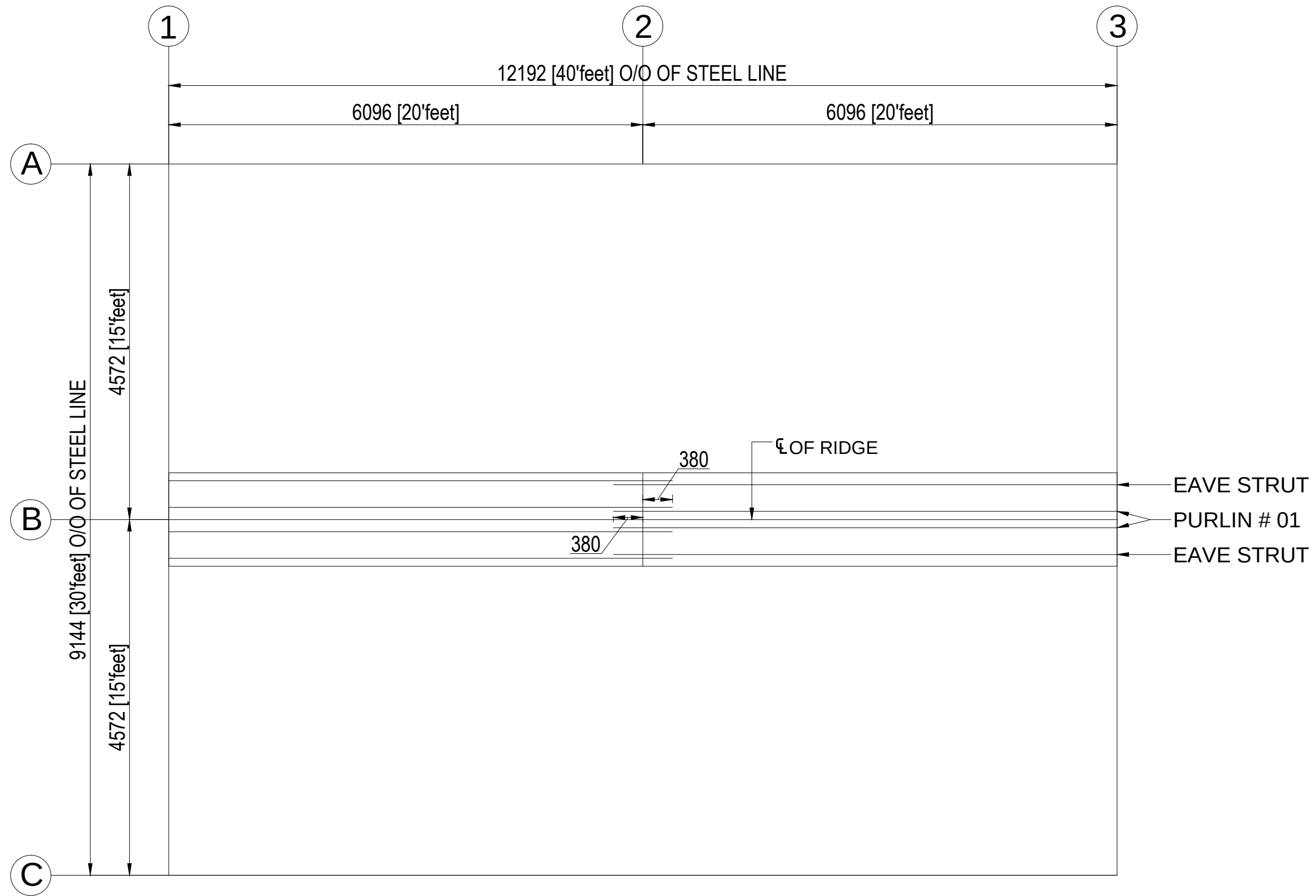
ROOF MONITOR FRAMING PLAN
